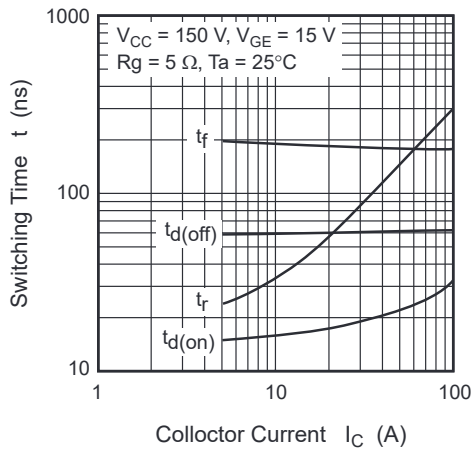
Switching Characteristics (Typical) (1)
