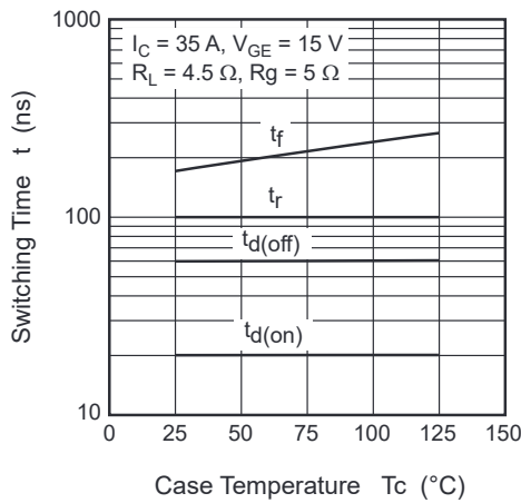
Switching Characteristics (Typical) (3)
